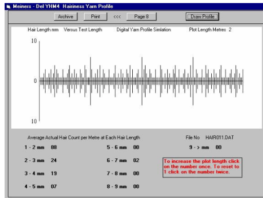
Yarn Hairiness Distribution Plot
